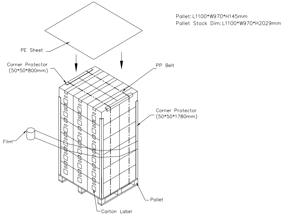
Figure. 9-2 Packing method
